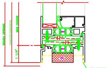
241 SILL 325 CASEMENT OUT BUTT HINGES
