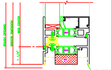
240 SILL 325 CASEMENT OUT 4-BAR ARMS
