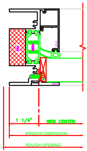
403 JAMB 325 PROJECT OUT \ FIXED
