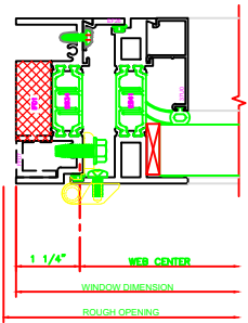
446 JAMB 325 FIXED \ CASEMENT OUT BUTT HINGES
