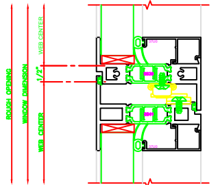
541 MEETING RAIL 325 FIXED \ CASEMENT OUT BUTT HINGES
