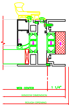
445 JAMB 325 FIXED \ CASEMENT OUT CAM LOCKS
