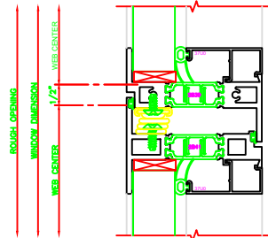
540 MEETING RAIL 325 FIXED \ CASEMENT OUT 4-BAR ARMS
